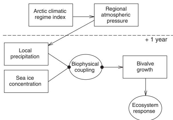
Fig. 8 Schematic representation of the Arctic Climate Cascade, where bivalve growth, and by inference, other ecosystem processes are linked to climatic forcing factors through variation in physical variables.
