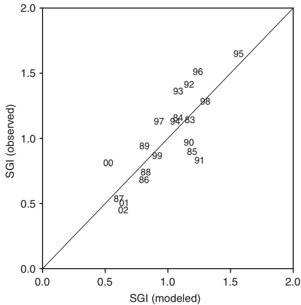
Fig. 6 Scatterplot of observed vs. modeled SGI from 1983 to 2002 with the growth years shown as data points. Line represents a perfect prediction by the model of actual growth rates of the Serripes groenlandicus population.
