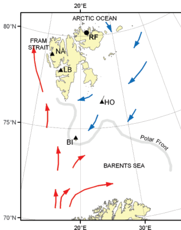
Fig. 1 Map of the study region showing the Spitsbergen Archipelago, general current patterns, the locations of the meteorological stations (BI, Bear Island, HO, Hopen, LB, Longyearbyen, NÅ, Ny Ålesund), and the collection site of Serripes groenlandicus (Rijpfjord, RF). The polar front is the average location of maximum ice cover in late winter.
