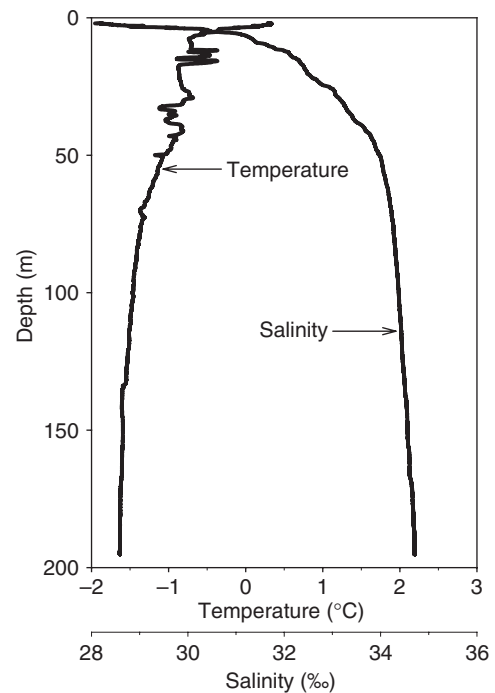
Fig. 2 Temperature and salinity profile from Inner Rijpfjord, near the location of bivalve collection, on 28 August 2003.
