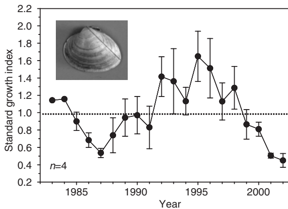
Fig. 4 Standard Growth Index (SGI) ( \pm 1 standard error of the mean) of the Serripes groenlandicus from Rijpfjord, Svalbard (Norway) collected live on 28 August 2003. Growth increments were calculated using external measurements and the von Bertalanffy equation to remove ontogenetic changes in growth. An SGI greater than 1.0 indicates greater than average growth while one less than 1.0 poorer than average. Growth was measured along the line indicated on the shell. The dark bands representing winter cessation of growth are visible on the shell.
