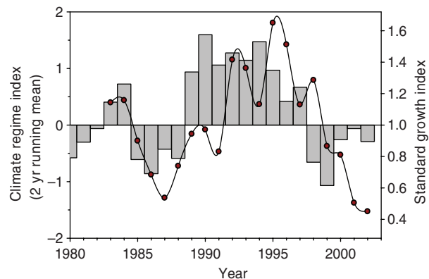
Fig. 5 Temporal patterns of the Arctic climate regime index (ACRI) (gray bars), lagged 1 year, and Serripes groenlandicus SGI (line). The ACRI data are 2-year running means of raw data, while the SGI data are untransformed.
