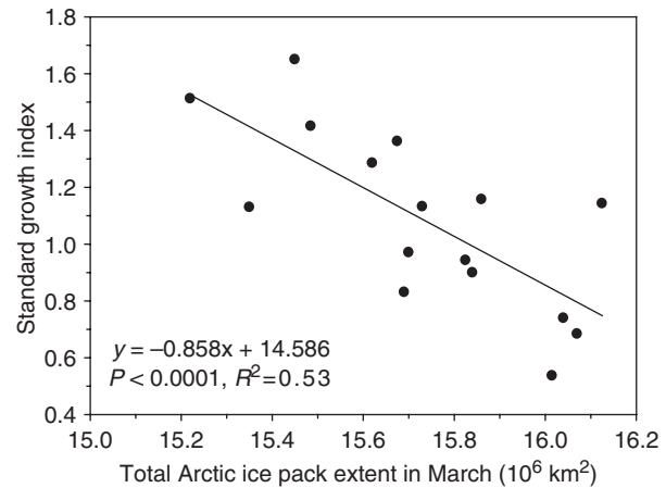
Fig. 7 Relationship between total Arctic-wide winter (March) sea ice extent (2-year running mean) and Serripes groenlandicus SGI from 1983 to 1998. (Ice data courtesy of National Snow and Ice Data Center, Boulder, CO, USA).
