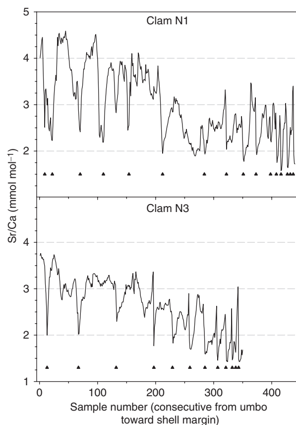
Fig. 3 Ratio of strontium to calcium in two Serripes groenlandicus shells (N1 and N3) from Rijpfjord. Samples were taken along each clam's height and are numbered from the umbo (sample number 0) to the ventral margin. Triangles correspond to the location of dark growth lines visible on a shell's exterior.
